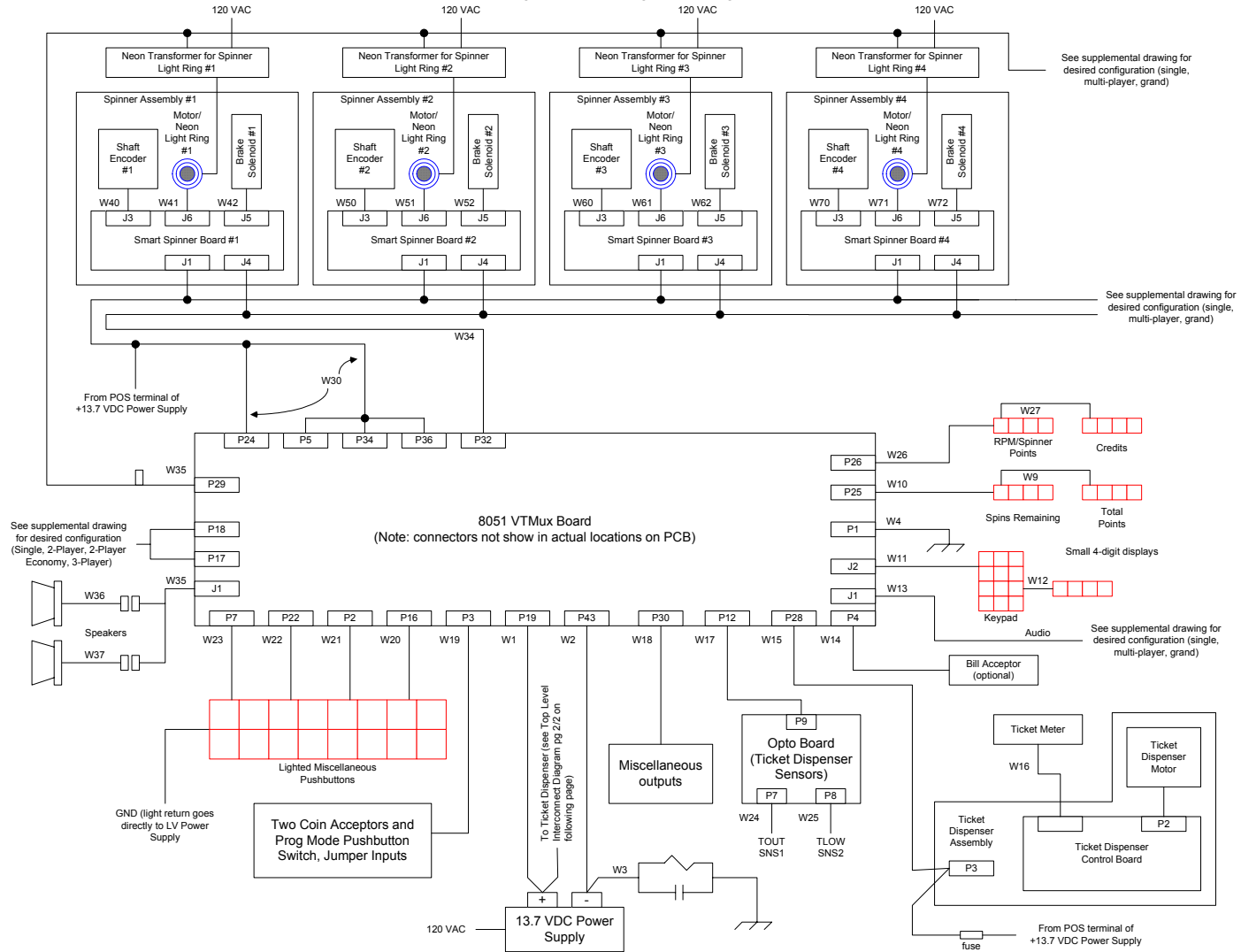
TOP LEVEL INTERCONNECT DIAGRAM
