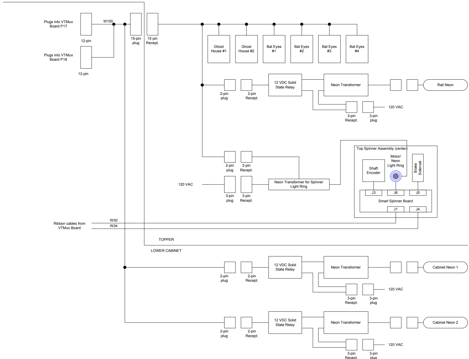
TOP SPINNER BLOCK DIAGRAM CENTER GAME
