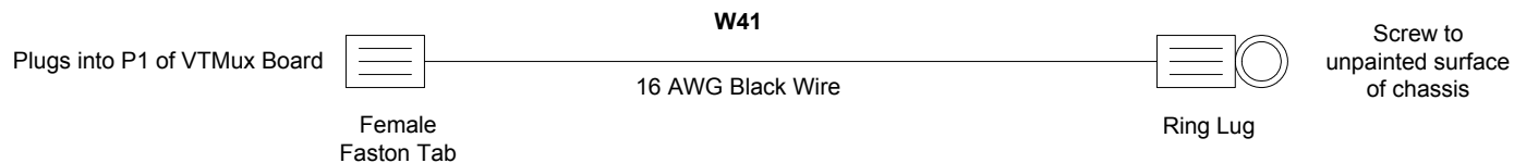
FIGURE 21 - AUDIO GROUND
