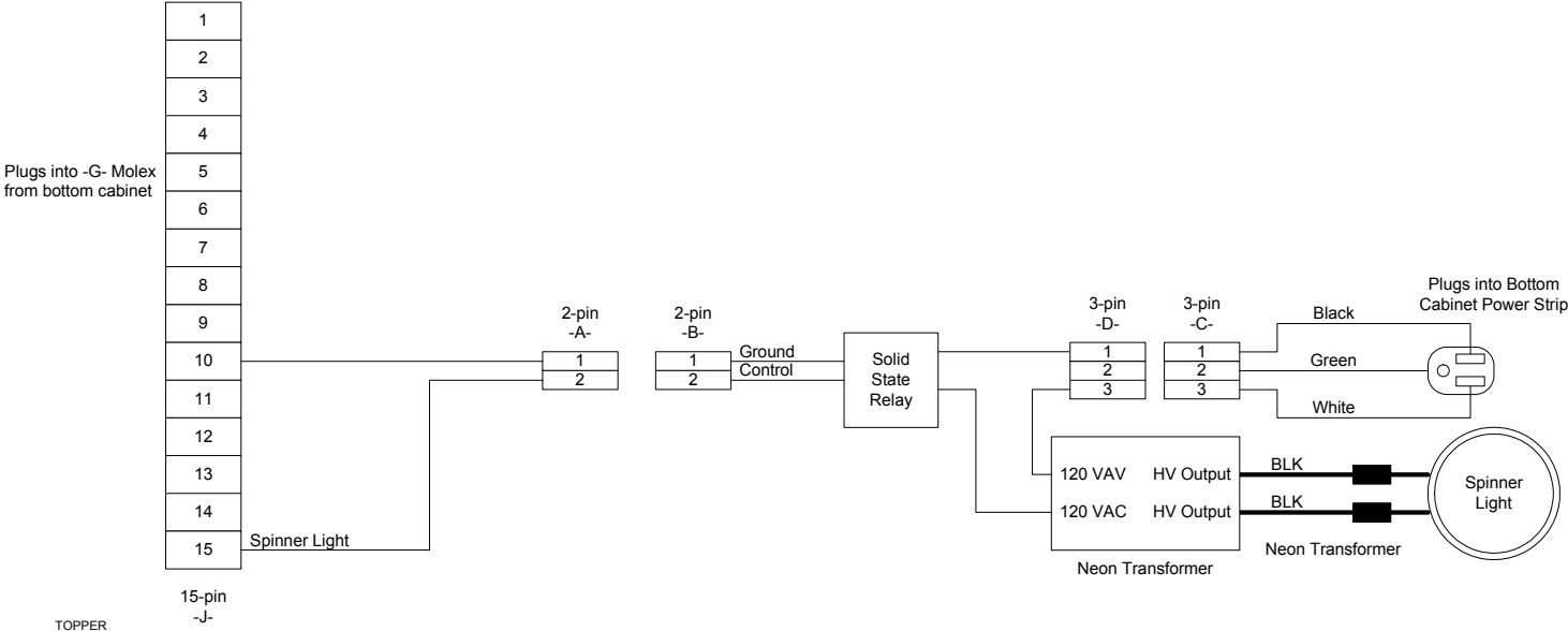
TOP SPINNER WIRING LEFT GAME
